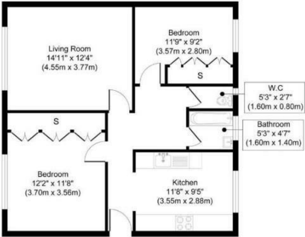
Floor Plan Approximate Floor Area 723.76 sq. ft (67.24 sq.m)
